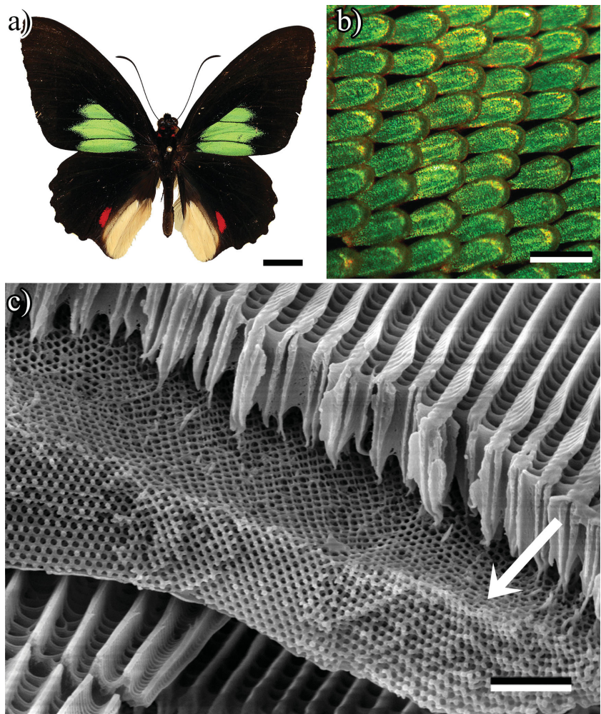
Figure 10. Biological gyroids, here in wing scales of the butterfly Parides sesostris . a) The butterfly (scale bar: 1 cm). b) The scales imbricating the wing (scale bar: 100 \mu\text{m} ). c) An electron micrograph of a cross section of the wing scale showing the gyroid structure and also highlighting the ridge and cross-ribs present on top of the gyroid photonic crystal (scale bar: 2 \mu\text{m} ). Reproduced with permission. 38 Copyright 2011, Royal Society.
