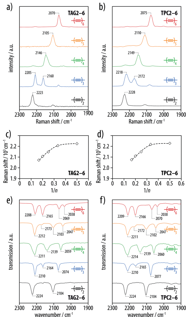
Fig. 3 IR and Raman spectra for the series of tetra-O-acetyl \beta -D-glucosyl oligoyne TAG2-6 and the corresponding tritylphenyl carboxylates TPC2-6. (a and b) Solid-state Raman spectra, (c and d) plots of the Raman band positions versus 1/n (the lines serve as guides to the eye), and (e and f) solid-state IR spectra of TAG2-6 and TPC2-6.
