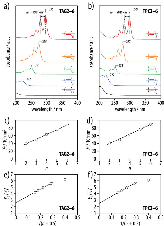
Fig. 2 (a) UV-vis spectra of the tetra-O-acetyl \beta -D-glucosyl oligoyne TAG2-6 in acetonitrile (concentrations in the range of c = 3.03 – 4.21 \mu\text{mol L}^{-1} ), and (b) of the corresponding tritylphenyl carboxylates TPC2-6 in cyclohexane (concentrations in the range of c = 5.86 – 6.55 \mu\text{mol L}^{-1} ). (c and d) Lewis-Calvin plots of the UV-vis absorption maxima of the two series with linear regressions with slopes of k = 12.2 \times 10^3 and 12.4 \times 10^3 \text{ nm}^2 ( R^2 = 0.996 and 0.991 ). (e and f) Plots of the energy of the optical transition versus 1/(n+0.5) , with the number of triple bonds n . An extrapolation of the linear regression to n = \infty yields values of 480 nm (2.6 eV) and 498 nm (2.5 eV), respectively, for the saturation wavelength of an infinitely long chain of conjugated triple bonds ( R^2 = 0.999 in both cases).
