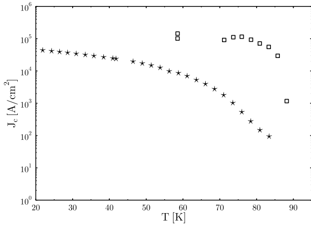
Fig. 4. Critical current density J_c of Batch 2 films as a function of temperature for \approx 100 nm thick Y123 films on \text{SrTiO}_3 ( \star ) and on \text{LaAlO}_3 ( \square ) substrates.
