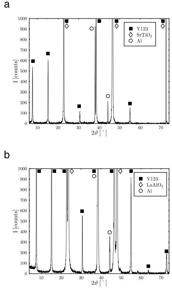
Fig. 7. \omega - 2\theta scan of Y123 samples from Batch 2 on \text{SrTiO}_3 (a) and on \text{LaAlO}_3 (b). Two of the peaks that arise neither from the Y123 nor from the substrate can be attributed to the (111) and (200) reflections of the aluminum sample support, which was accidentally exposed to the 1 cm wide line focus of the primary beam.
