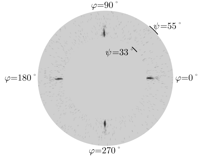
Fig. 8. Texture scan ( \varphi - \psi scan) of the Y123-{104} reflections of a Batch 2 sample on SrTiO 3 . The elongated peak shape is a consequence of the X-ray beam profile ( 1 \times 10 mm 2 line focus).
